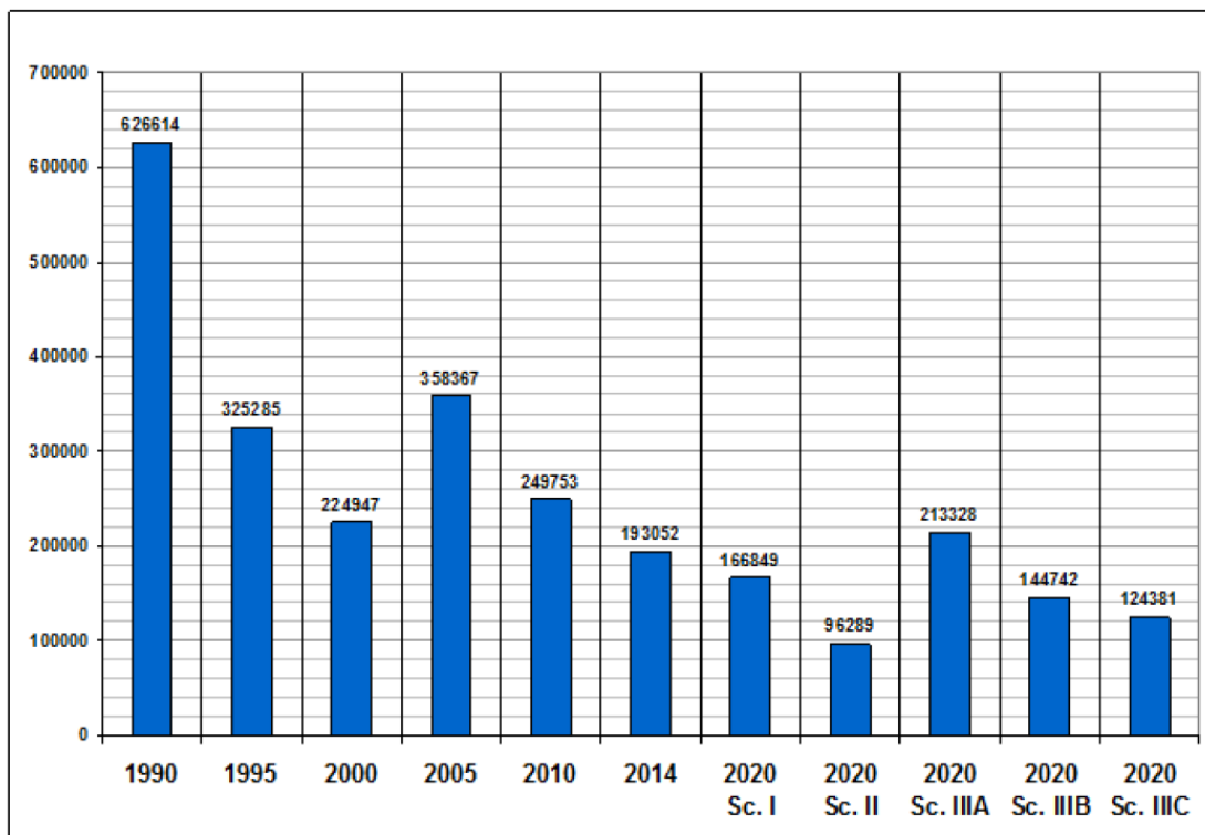
Fig. 6. Reconstruction in the period 1990-2014 and projected emissions (t) of oxides of nitrogen (NOx) from road vehicles on the territory of Ukraine under different scenarios of socio-economic development and public regulation Resource: (Study of the impact on emissions..., 2015)
