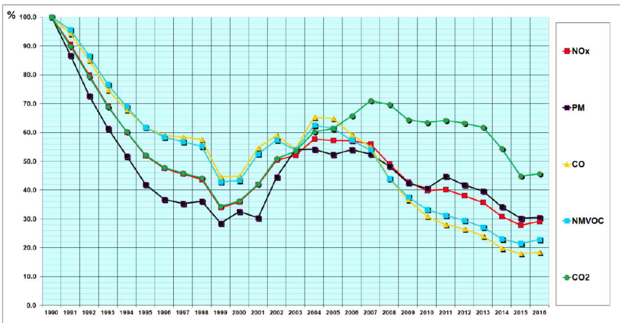
Fig. 5. Reconstruction by methods of mathematical simulation of emissions from road vehicles on the territory of Ukraine of carbon dioxide (CO2), nitrogen oxides (NOx), particulate matter (PM2.5), carbon monoxide (CO) non-methane volatile organic compounds (NMVOC) Resource: (Study of the impact on emissions..., 2016)
